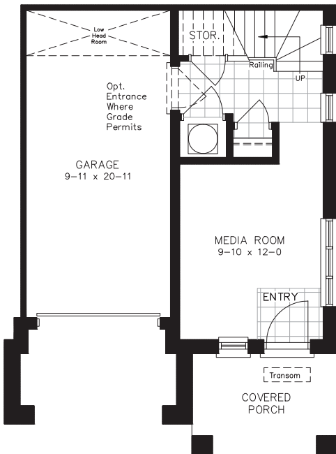
END UNIT - GROUND FLOOR - G1
