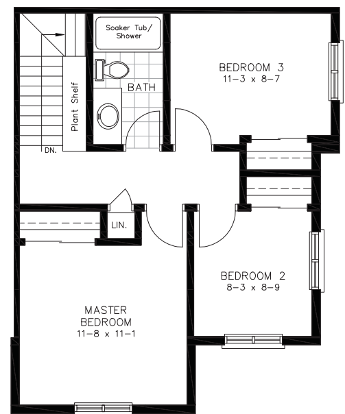
END UNIT - SECOND FLOOR - S1
