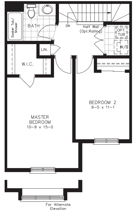
END UNIT - SECOND FLOOR - S1
